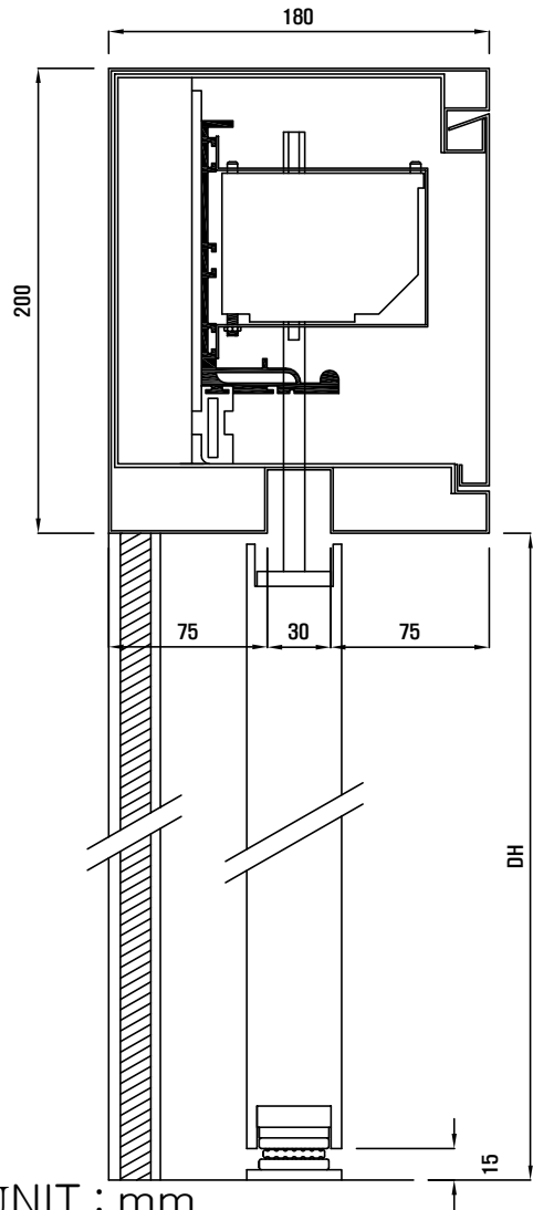
VERTICAL SECTION
