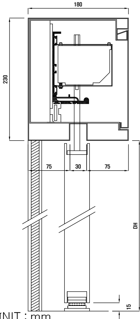
VERTICAL SECTION
