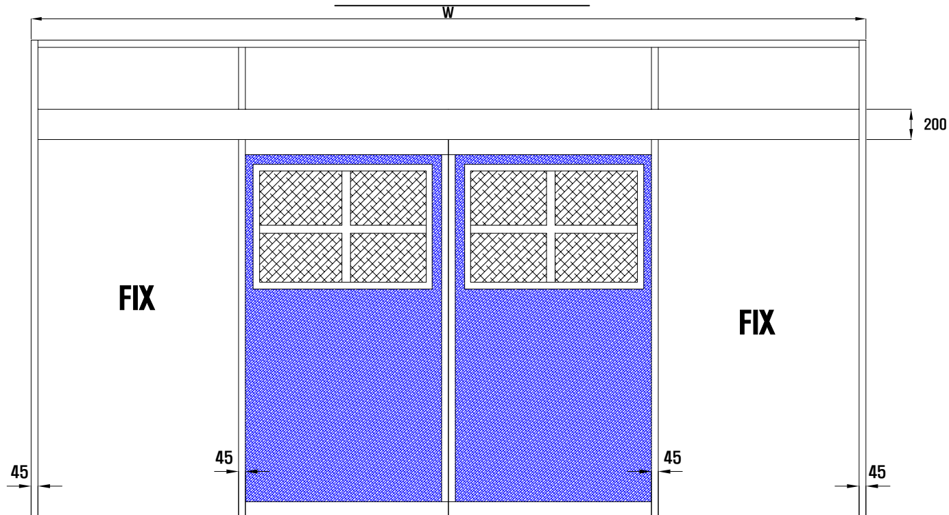
ELEVATION SECTION
